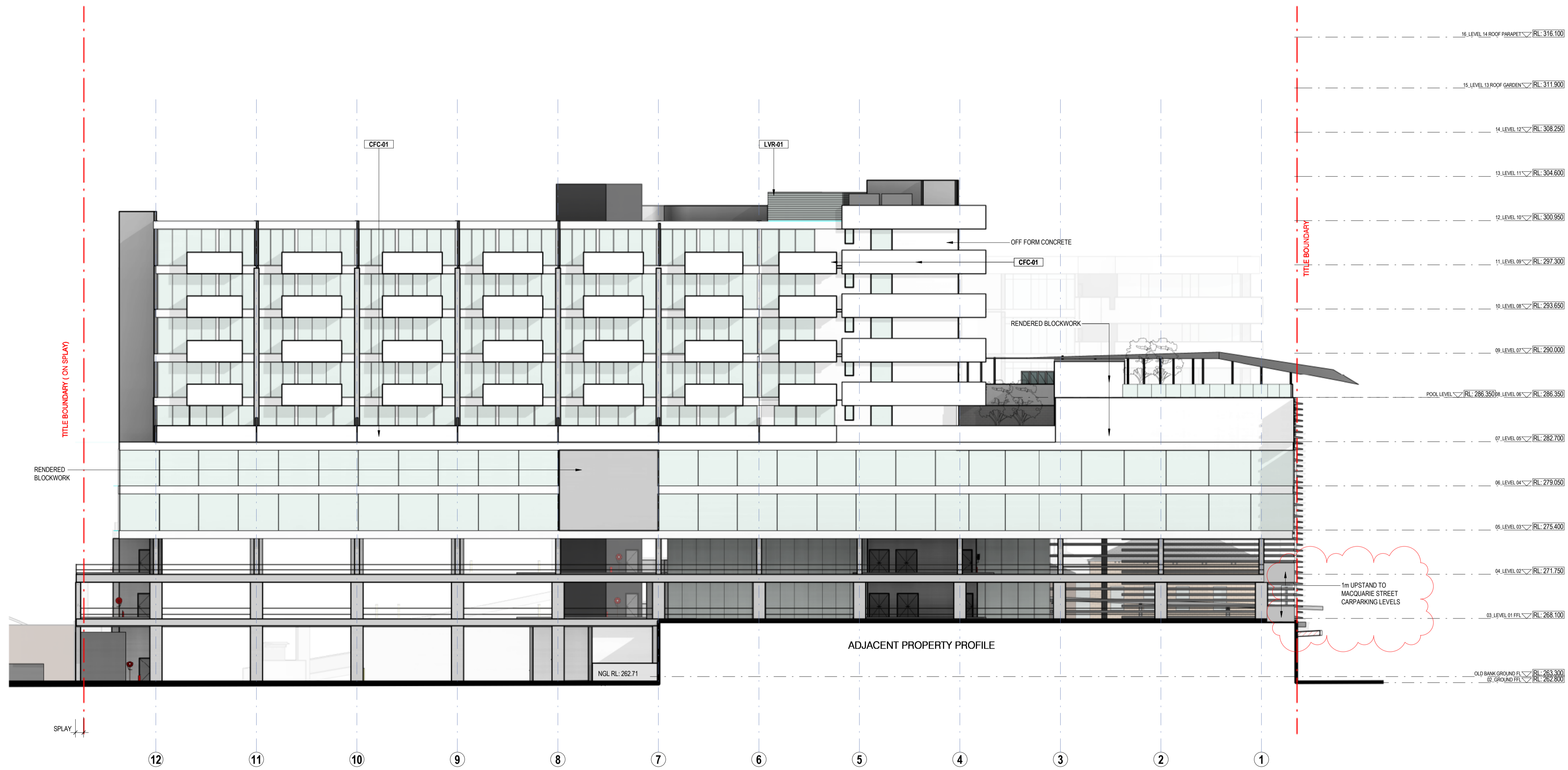
(5) PROPOSED NORTH EAST ELEVATION 1 : 200
